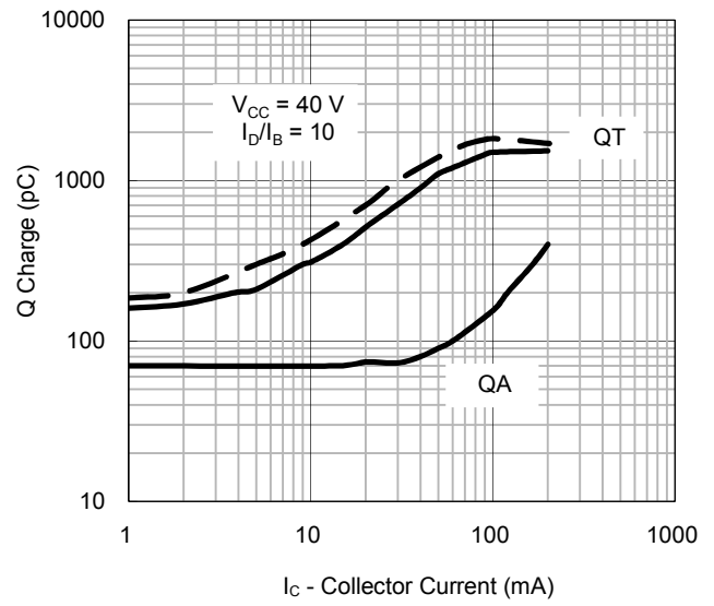
Fig.2 Charge Data
