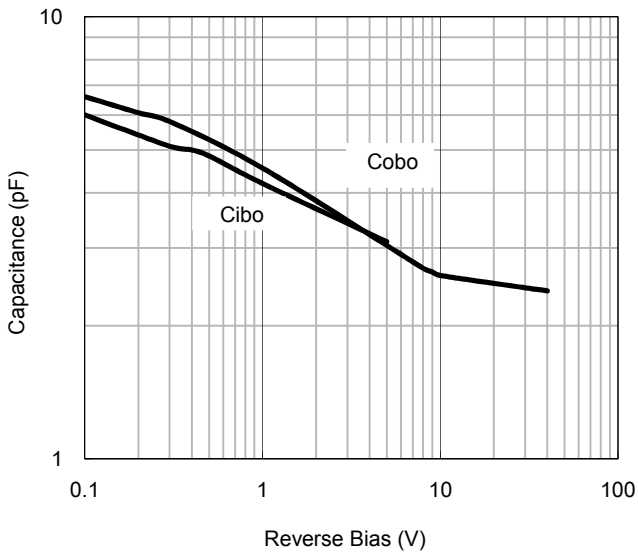
Fig.1 Capacitance
